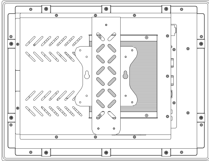
c-1. FP8151 Wall mounting dimension
